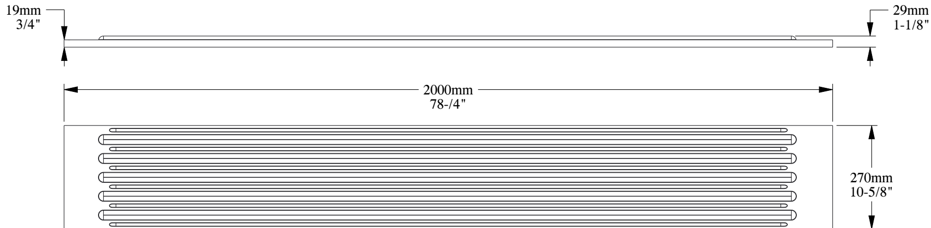
SCALE 1:10
